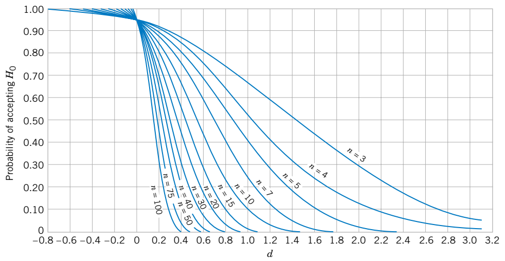
Chart VII Operating Characteristic Curves (continued)
