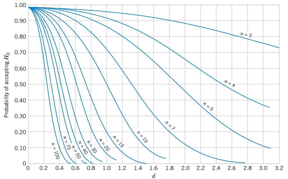
(f) O.C. curves for different values of n for the two-sided t -test for a level of significance \alpha = 0.01 .
