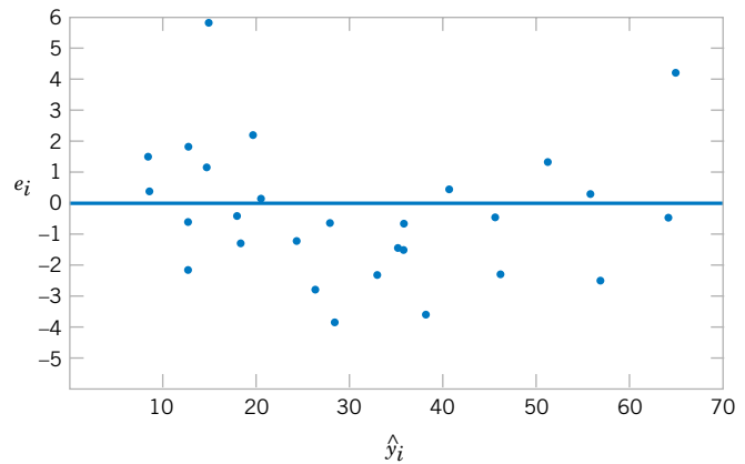
Figure 12-7 Plot of residuals against \hat{y}_i .
