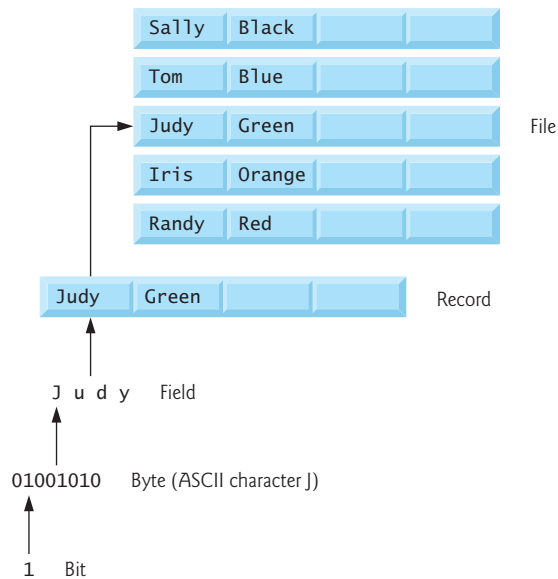
Fig. 11.1 | Data hierarchy.
