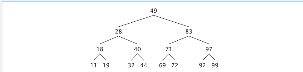
Fig. 12.22 | A 15-node binary search tree.
