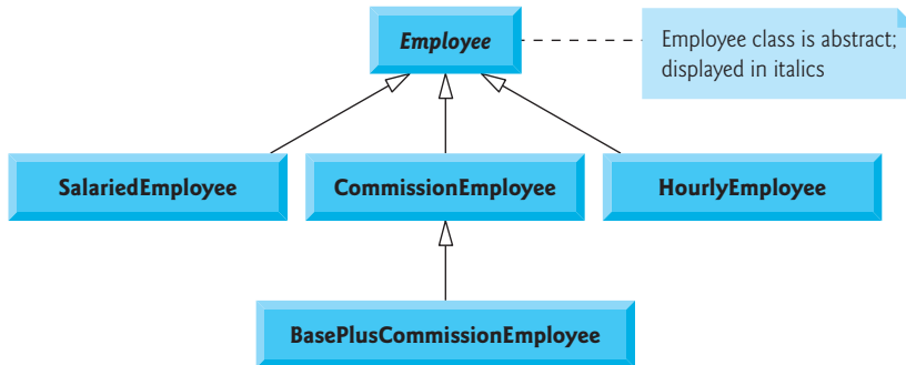
Fig. 21.11 | Employee hierarchy UML class diagram.
