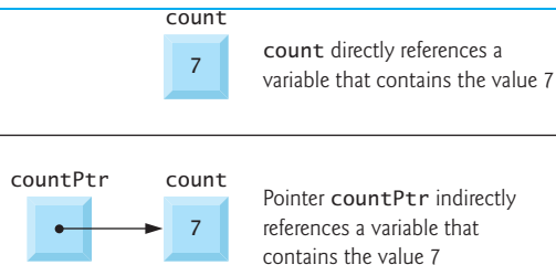
Fig. 7.1 | Directly and indirectly referencing a variable.
