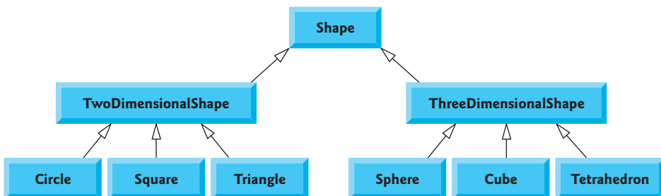
Fig. 20.3 | Inheritance hierarchy for Shapes.
