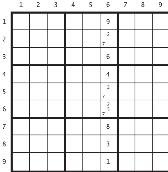
Fig. D.4 | Notation showing the complete sets of possible values for open cells.
