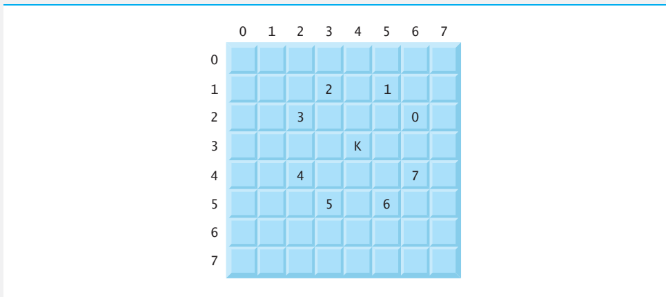
Fig. 6.25 | The eight possible moves of the knight.
