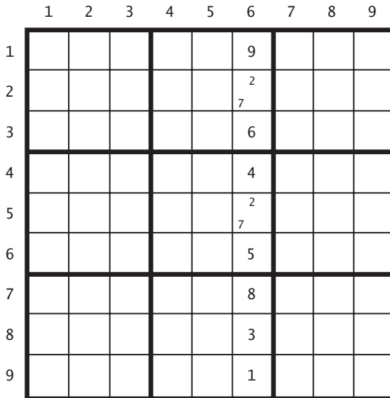
Fig. D.5 | Committing cell s[6][6] to the singleton value 5.
