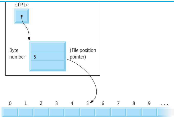
Fig. 11.14 | File position pointer indicating an offset of 5 bytes from the beginning of the file.
