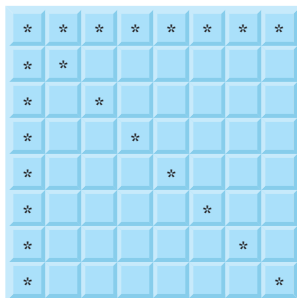
Fig. 6.26 | The 22 squares eliminated by placing a queen in the upper-left corner.
