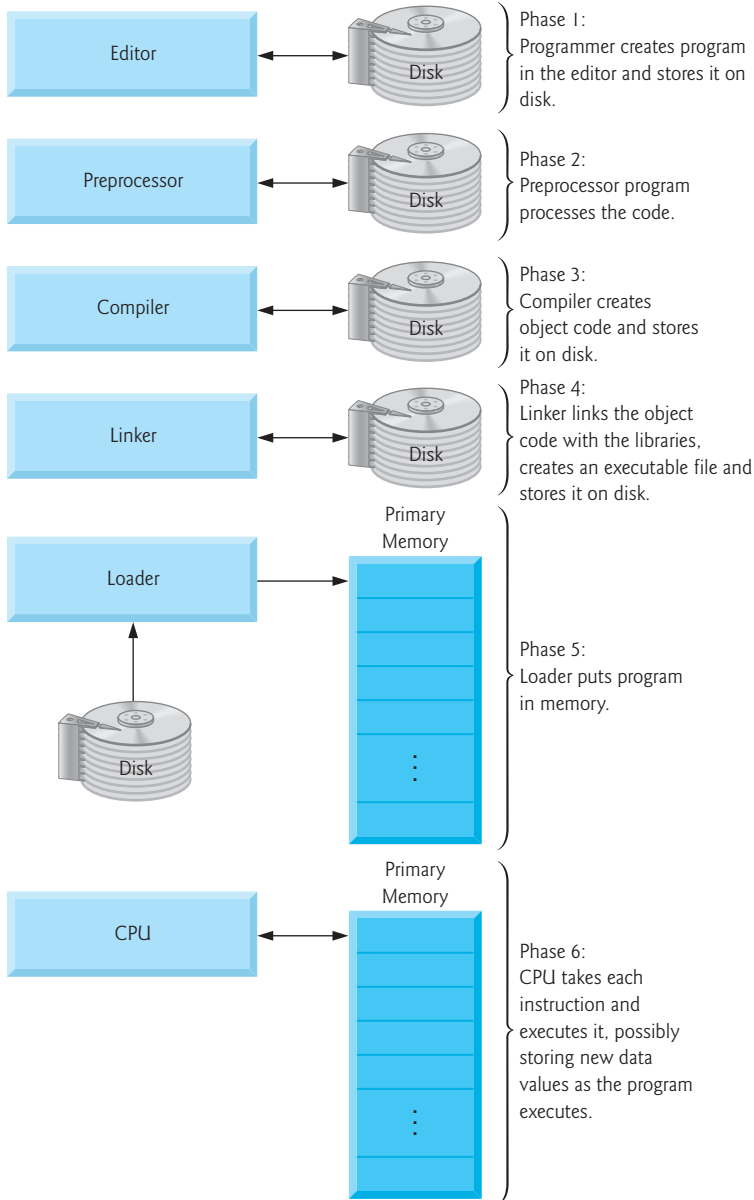
Fig. I.1 | Typical C development environment.
