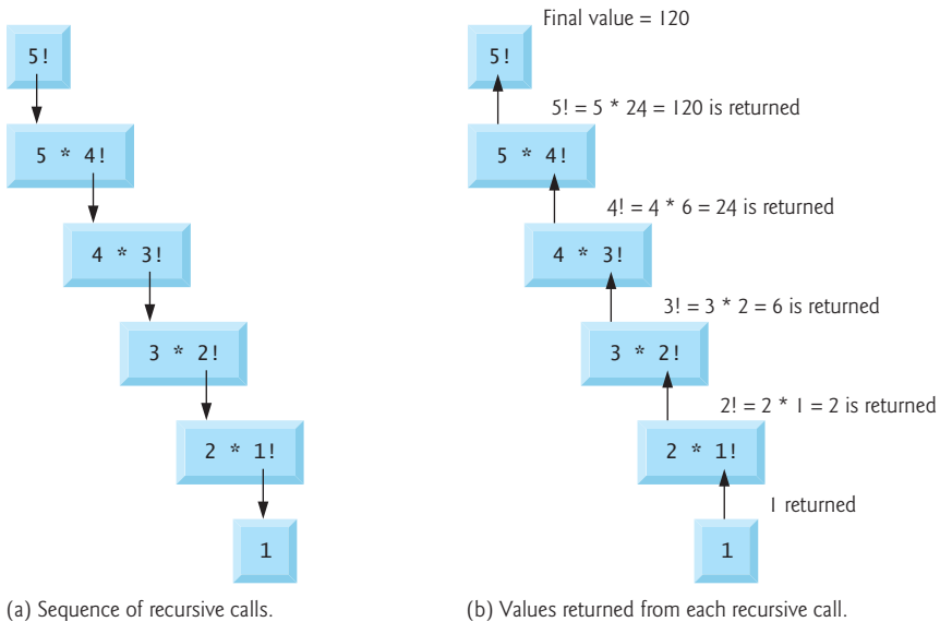
Fig. 5.13 | Recursive evaluation of 5! .
