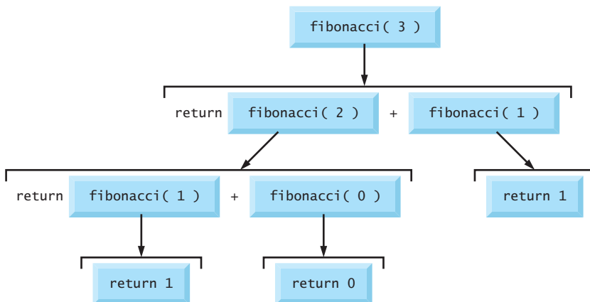
Fig. 5.16 | Set of recursive calls for fibonacci(3) .
