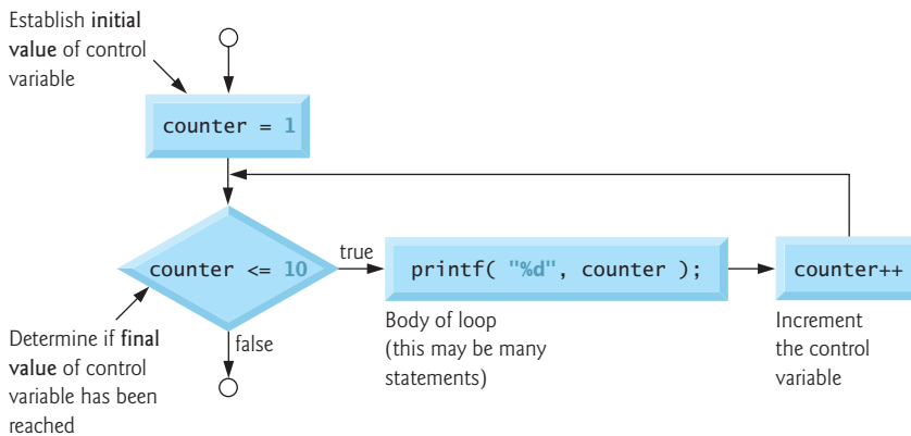
Fig. 4.4 | Flowcharting a typical for repetition statement.
