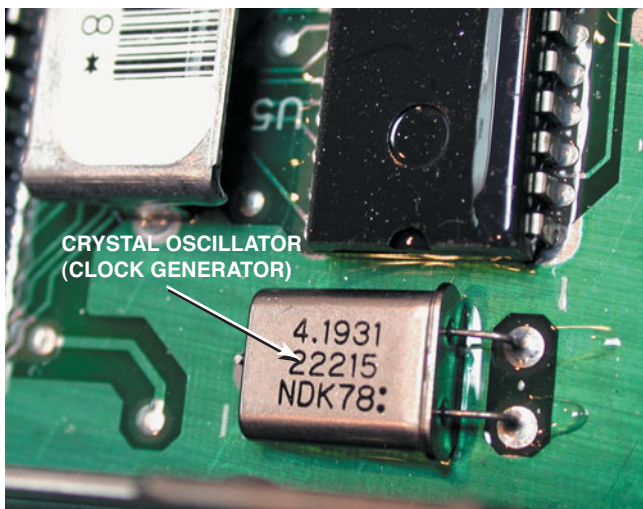
FIGURE 71-6 The clock generator produces a series of pulses that are used by the microprocessor and other components to stay in step with each other at a steady rate.
