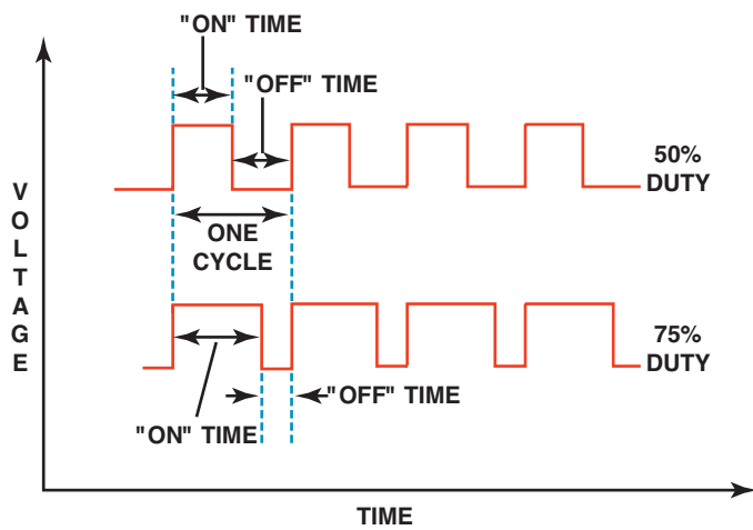
FIGURE 71-12 Both the top and bottom pattern have the same frequency. However, the amount of on-time varies. Duty cycle is the percentage of the time during a cycle that the signal is turned on.
