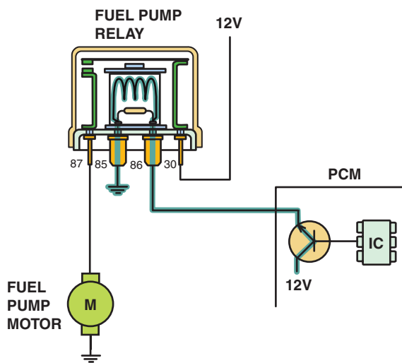
FIGURE 71-9 A typical output driver. In this case, the PCM applies voltage to the fuel pump relay coil to energize the fuel pump.
