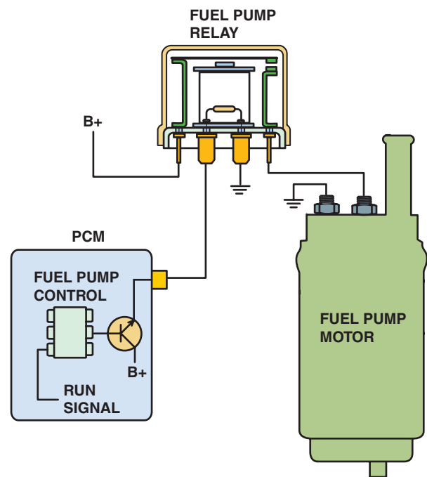
FIGURE 71-11 A typical module-controlled high-side driver (HSD) where the module itself supplies the electrical power to the device. The logic circuit inside the module can detect circuit faults including continuity of the circuit and if there is a short-to-ground in the circuit being controlled.
