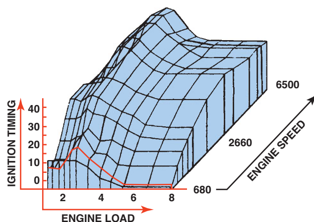
FIGURE 71-5 Typical engine map developed from testing and used by the vehicle computer to provide the optimum ignition timing for all engine speeds and load combinations.
