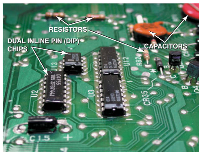
FIGURE 71-4 Many electronic components are used to construct a typical vehicle computer including chips, resistors, and capacitors.
