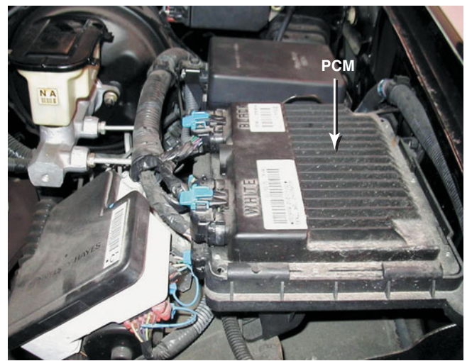
FIGURE 71-7 This powertrain control module (PCM) is located under the hood on this Chevrolet pickup truck.
