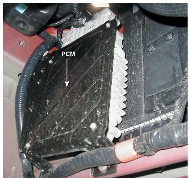
FIGURE 71-8 This PCM on a Chrysler vehicle can only be seen by hoisting the vehicle, because it is located next to the radiator and in the airflow to help keep it cool.
