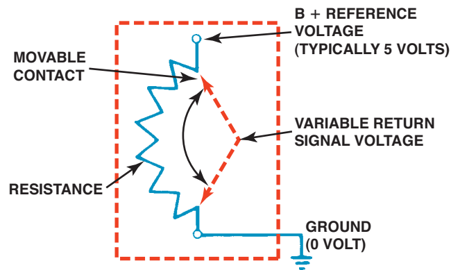
FIGURE 71-2 A potentiometer uses a movable contact to vary resistance and send an analog voltage right to the PCM.
