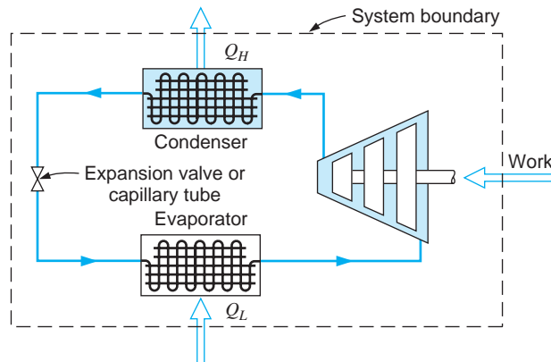
FIGURE 7.6 A simple refrigeration cycle.
