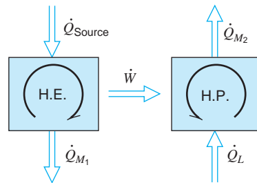
FIGURE 12.22 A heat engine–driven heat pump or refrigerator.
